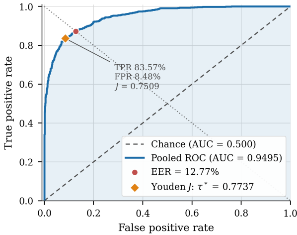
Fig. 4. Left: pooled ROC over all 2,240 leave-one-subject-out verification pairs, with the equal-error point and the Youden-optimal point \tau^* = 0.7737 marked. Right: paired change in ROC-AUC against the deployed model for each ablation variant, with 95% confidence intervals; every interval lies wholly below zero.
