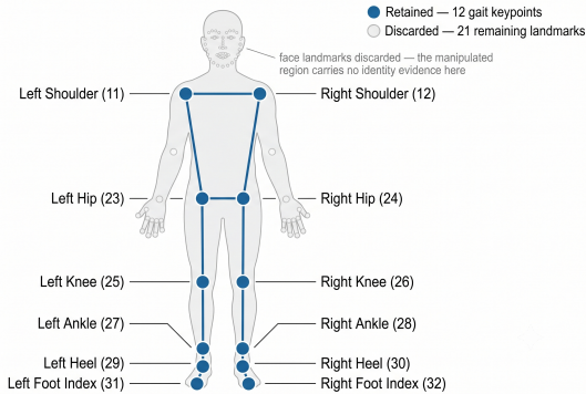
Fig. 3. The 12 retained gait keypoints (blue) of the 33 MediaPipe landmarks; facial, elbow and wrist landmarks are discarded.
