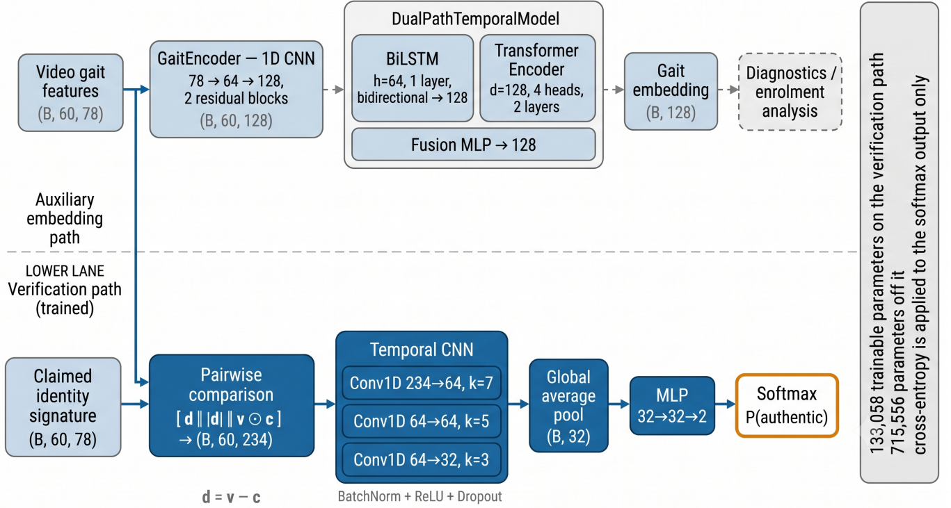
Fig. 4. Network architecture as trained. The lower lane is the verification path: the observed and claimed sequences are combined into a 234-channel per-timestep comparison tensor, passed through a three-layer temporal CNN, pooled and classified. The upper lane—a residual 1D CNN encoder feeding a parallel BiLSTM and Transformer—produces a 128-dimensional gait embedding used for enrolment analysis and diagnostics. The two lanes do not join: under the cross-entropy objective applied to the softmax output, 133,058 parameters lie on the verification path and 715,556 do not. Section III-F states the consequences of this separation, and Section VII-C treats it as a threat to validity.
