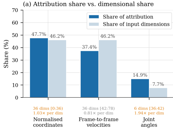
Fig. 5. Share of attribution against share of input dimensions for each feature block. Joint angles occupy 7.69% of the input but draw 14.92% of attribution, a per-dimension ratio of 1.94.
