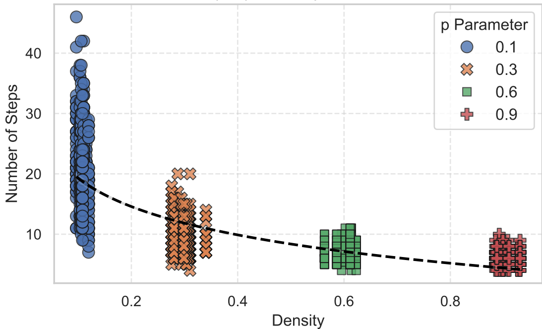
G(n,p) : Density vs Steps
