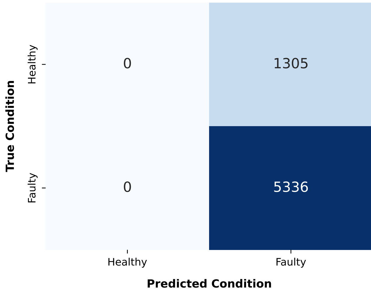
Confusion Matrix: Fusion Model (NLN-EMP Test Set)
