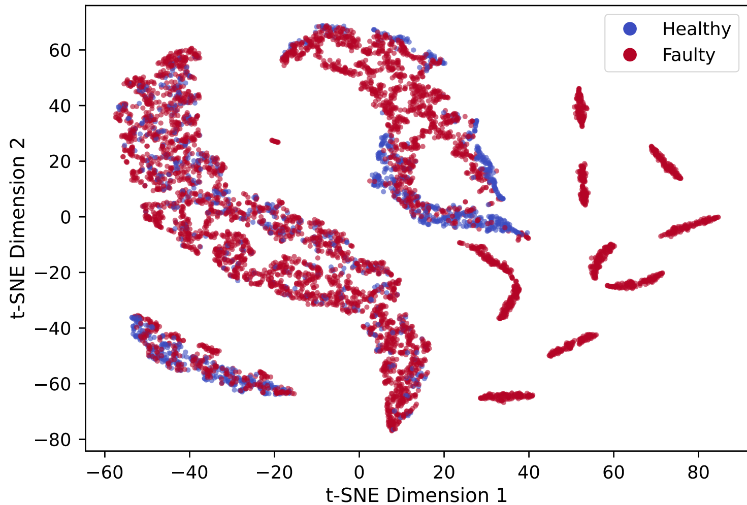
t-SNE Feature Visualization (Full Test Set)
