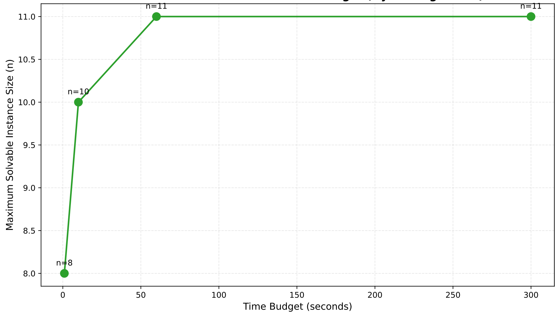
Maximum Instance Size vs. Time Budget (Hybrid Algorithm)
