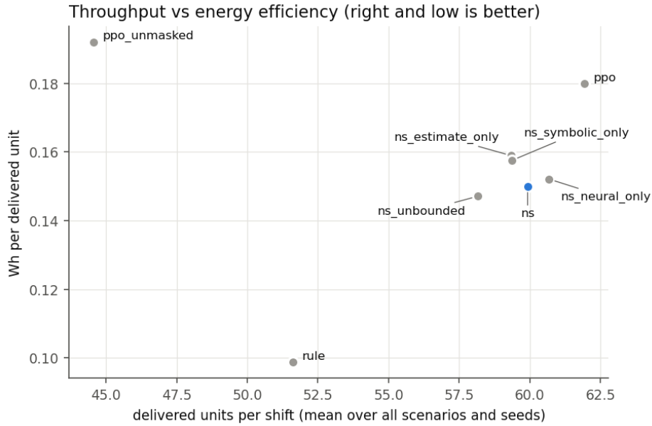
Figure 7.3: Delivered units against energy per delivered unit, averaged over all scenarios and seeds. Points towards the lower right deliver more for less energy.
