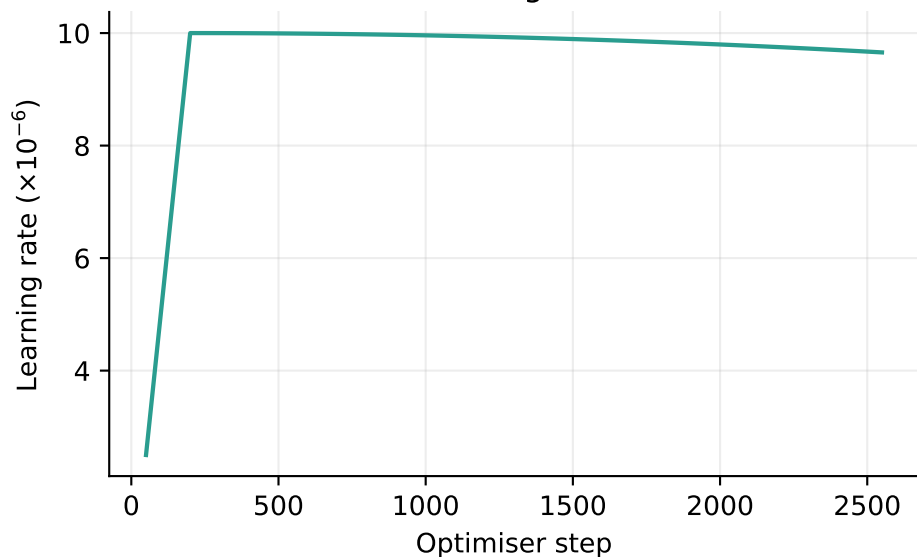
Executed learning-rate schedule
