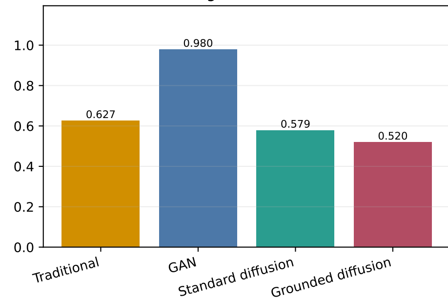
Aligned SSIM ↑
