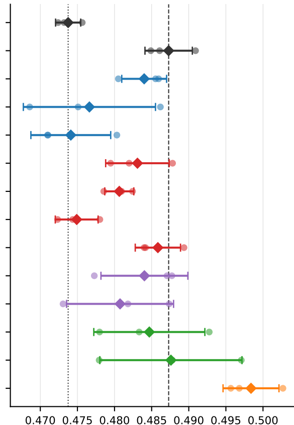
CompBench, averaged checkpoints
