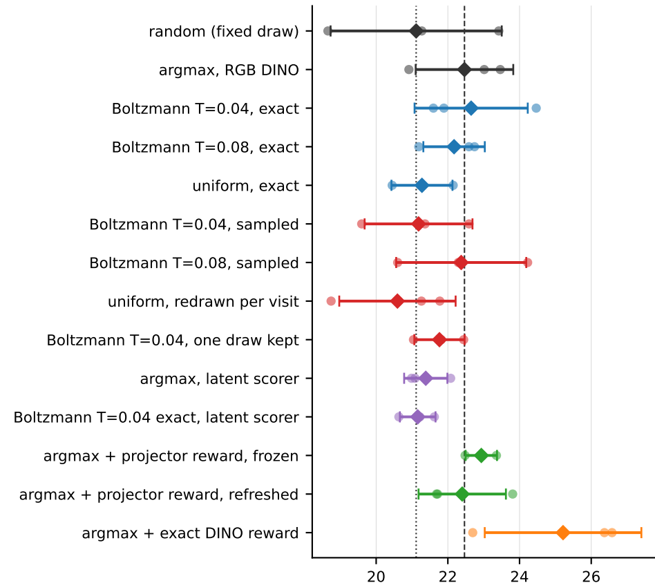
GenEval2 x100, raw final
