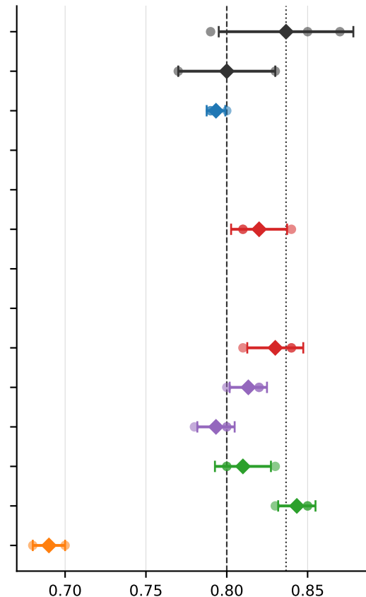
CMMD, averaged (lower is better)
