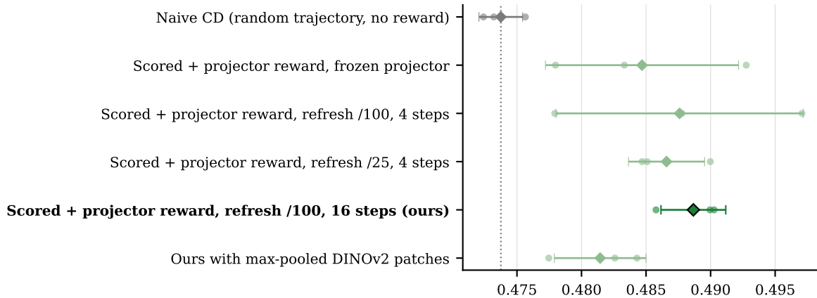
T2I-CompBench (mean of 8 categories)
