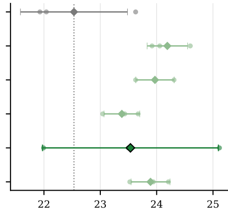
GenEval2 ( \times 100 )
