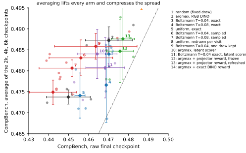
Figure 6: Raw final against averaged CompBench per arm. Averaging lifts every arm by 0.01 to 0.03 and shrinks the differences between them; the arms that gain most are those whose final iterate wanders most.
