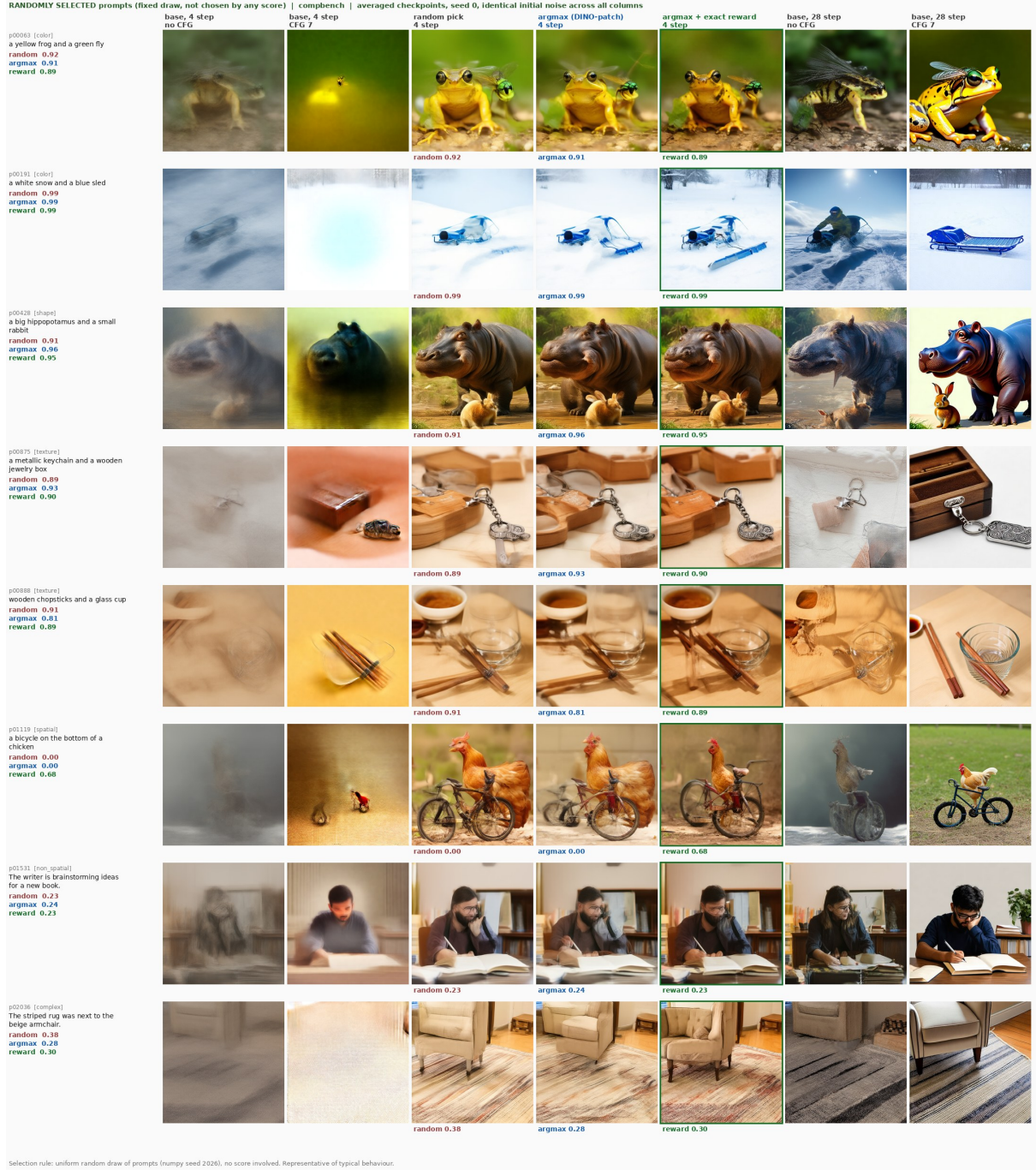
Figure 18: Eight T2I-CompBench prompts drawn uniformly at random (numpy seed 2026), no score involved; same columns and models as Figure 16.
