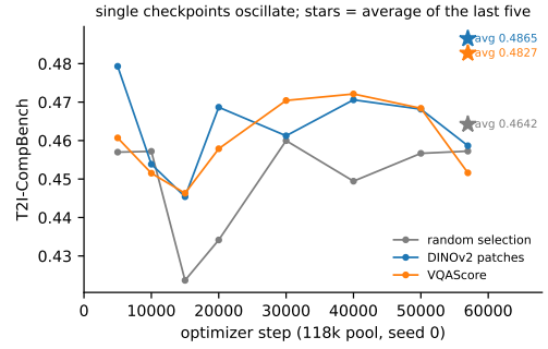
Figure 7: CompBench of every saved checkpoint of the seed-0 118k runs; the star marks the weight average of the last five checkpoints of each arm (Section 10.4).
