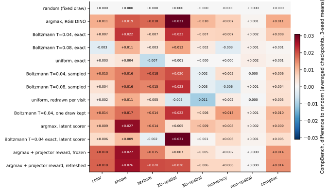
Figure 5: CompBench per category, averaged checkpoints, three-seed means, as differences to the random arm. The scored arms gain on colour, shape, spatial and numeracy and not on non-spatial, whose CLIPScore evaluator does not separate students.
