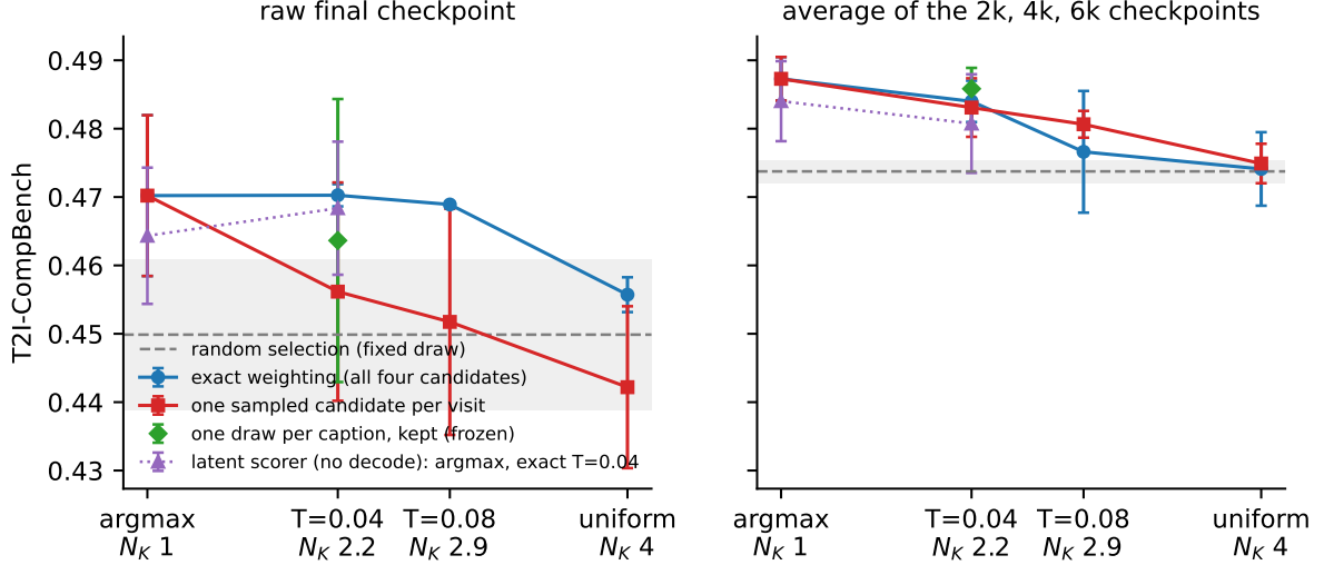
Figure 9: CompBench of the selection rules as a function of the Kish count of their weights, raw final checkpoints (left) and the average of the 2k, 4k and 6k checkpoints (right). Points are seed means, bars are seed standard deviations, the grey band is the random baseline. On raw checkpoints the sampled arms fall away from argmax while the exact arms stay flat; after identical averaging the two estimators coincide and the ordering follows the weight on the best candidate.
