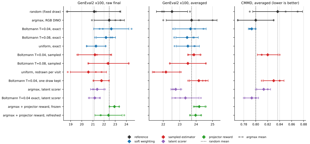
Figure 2: The same arms on GenEval2 (raw final and averaged checkpoints) and on CMMD (averaged checkpoints, lower is better). GenEval2 does not separate any two arms at three seeds; CMMD is within 0.03 for every scored arm after averaging.
