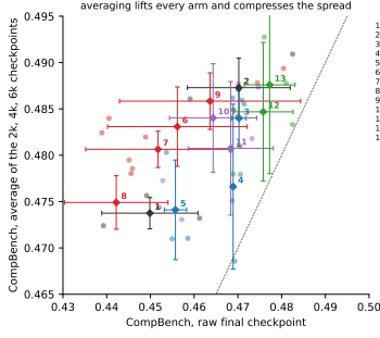
Figure 4: Raw final against averaged CompBench per arm. Averaging lifts every arm by 0.01 to 0.03 and shrinks the differences between them; the arms that gain most are those whose final iterate wanders most.
