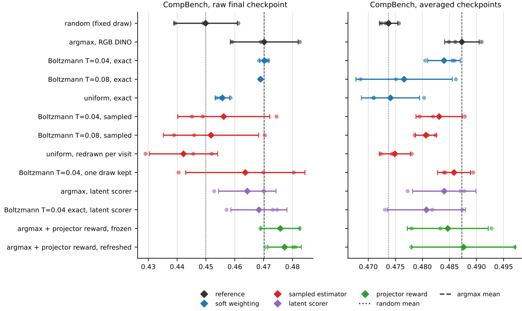
Figure 1: All arms trained on the 3k pool with the 3k configuration, three seeds each: CompBench seed values (dots), mean and standard deviation (diamond, bar), on raw final and on averaged checkpoints. Dotted and dashed lines are the random and argmax means. Colours group the arms by the choice they vary in Table 6.
