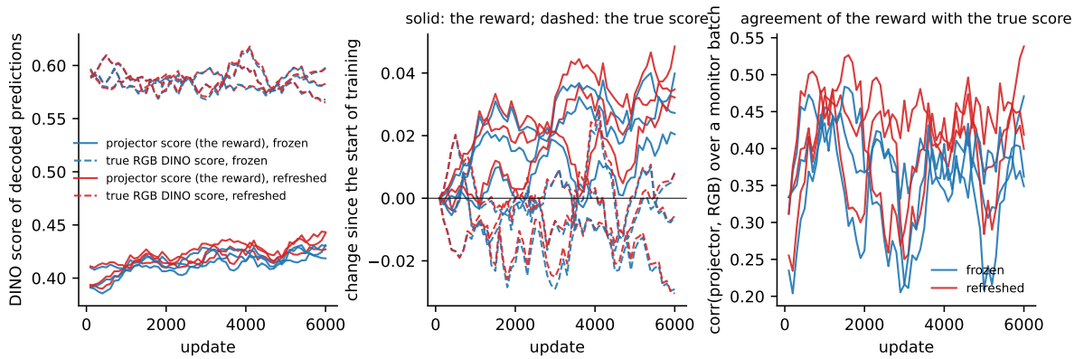
Figure 10: The hacking monitor of the six reward runs. Left: projector score (solid) and true RGB score (dashed) of the same decoded predictions over training. Middle: their change since update 100. Right: correlation between the two over each monitor batch. The reward rises in every run; the RGB score does not follow.
