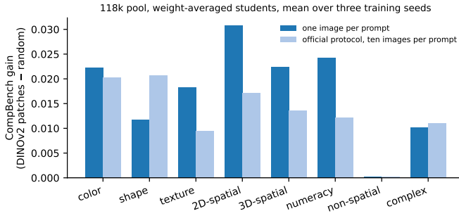
Figure 6: Per-category CompBench gain of DINOv2 patch selection over random selection at 118k (three-seed means of the averaged students) under both protocols. The gain is spread over the attribute-binding, spatial and counting categories and is zero on non-spatial, whose CLIPScore evaluator does not separate any two students in this work.
