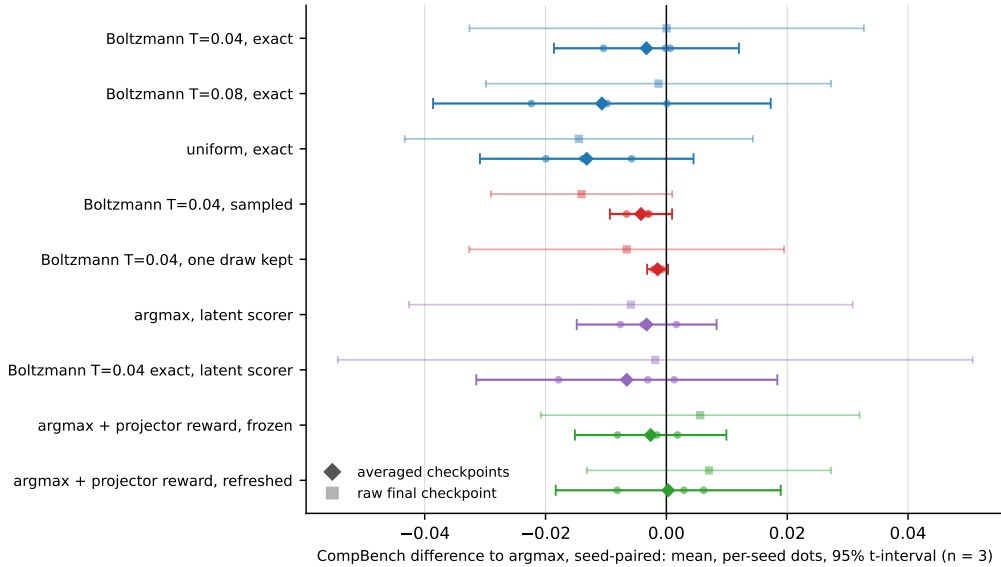
Figure 3: Seed-paired CompBench difference of every arm to argmax on averaged checkpoints (diamonds, with per-seed dots and 95% t -intervals) and on raw final checkpoints (faint squares). Intervals that cross zero are “no detected difference”; three seeds resolve about 0.01.
