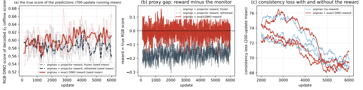
Figure 13: The exact reward against the projector rewards, in training. (a) The offline RGB DINO score of the decoded predictions (the hacking monitor, 32 latents every 100 updates, 700-update running mean; bold is the seed mean). (b) The reward seen by the optimizer minus that monitor: for the exact reward the two are the same quantity up to the resize path (correlation 0.9997); for the projector arms the gap is -0.19 and the two move apart. (c) The consistency loss of the exact-reward arm against argmax without a reward, 200-update means.
