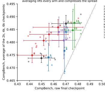
Figure 6: Raw final against averaged CompBench per arm. Averaging lifts every arm by 0.01 to 0.03 and shrinks the differences between them; the arms that gain most are those whose final iterate wanders most.
