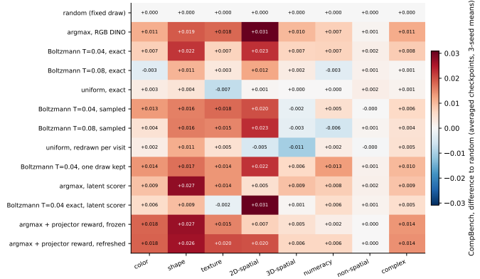
Figure 7: CompBench per category, averaged checkpoints, three-seed means, as differences to the random arm. The scored arms gain on colour, shape, spatial and numeracy and not on non-spatial, whose CLIP-Score evaluator does not separate students.
