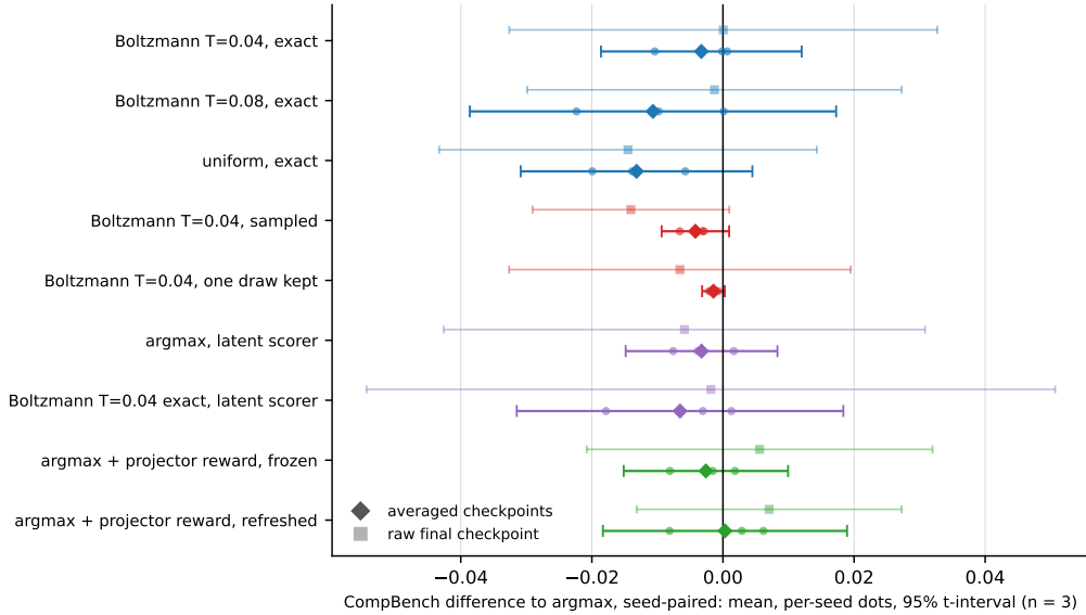
Figure 5: Seed-paired CompBench difference of every arm to argmax on averaged checkpoints (diamonds, with per-seed dots and 95% t -intervals) and on raw final checkpoints (faint squares). Intervals that cross zero are “no detected difference”; three seeds resolve about 0.01.
