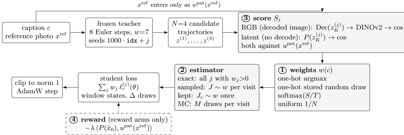
Figure 1: One training update. Every arm follows this flow; the four numbered blocks are the only places where arms differ (Table 6). The reference photograph enters only through its DINOv2 embedding, in the score and, in the reward arms, in the reward.
