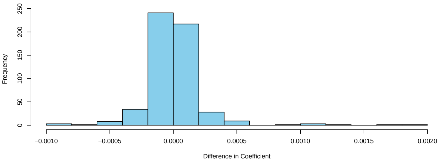
Difference between Neuron 234 and Concatenated Model with Interaction Terms
