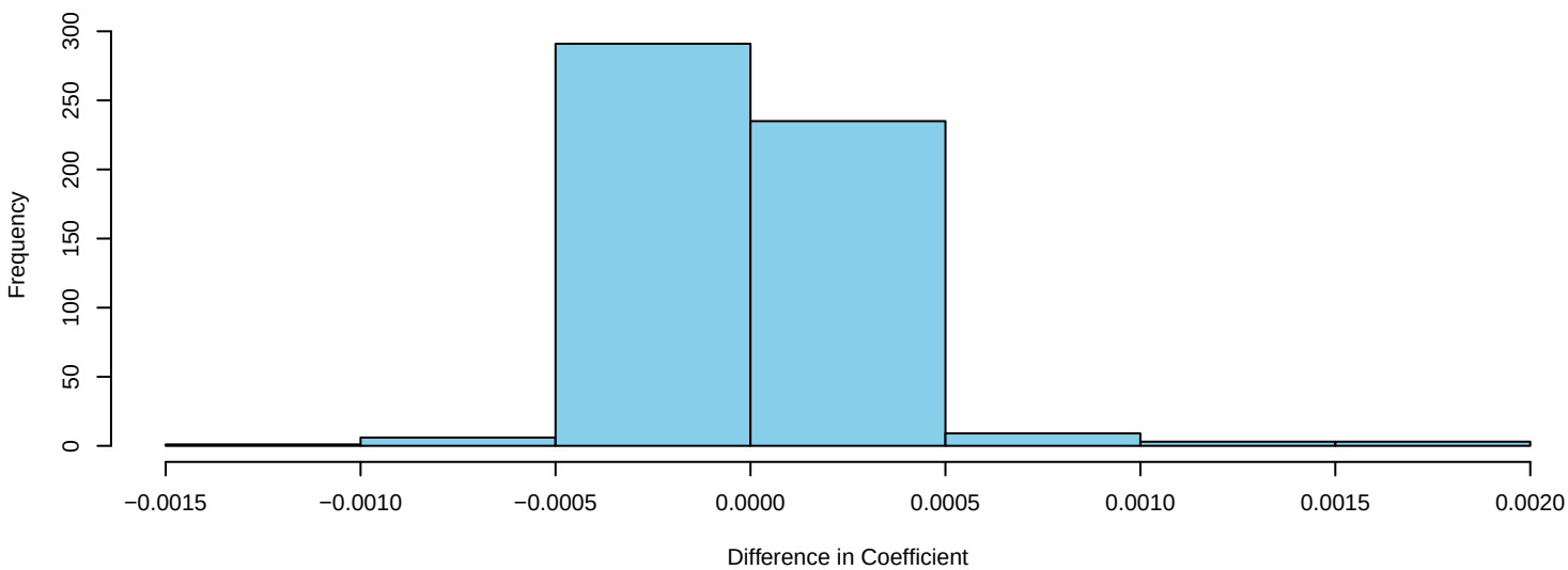
Difference between Neuron 281 and Concatenated Model with Interaction Terms
