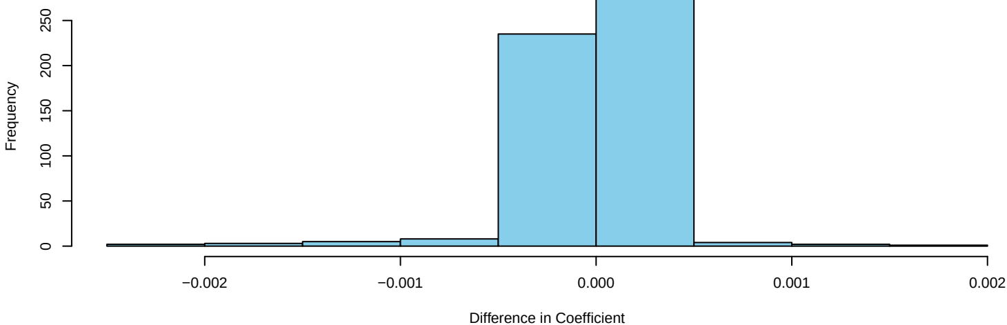
Difference between Neuron 281 and Concatenated Model with Interaction Terms
