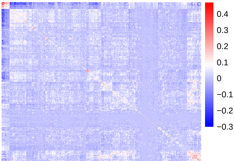
Pearson Correlation Heatmap
