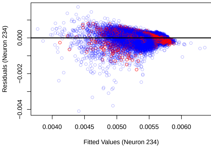
Residuals Plot for Neuron 234
