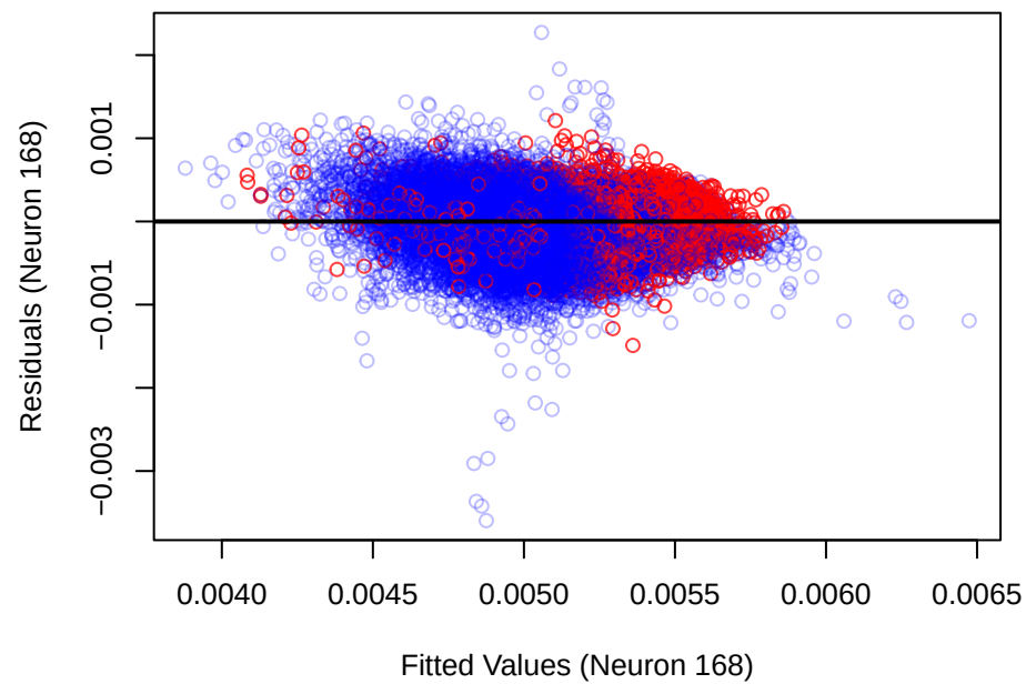
Residuals Plot for Neuron 168
