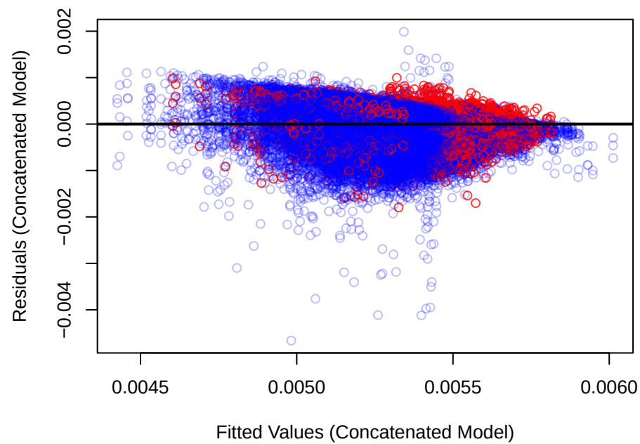
Residuals Plot for Concatenated Model
