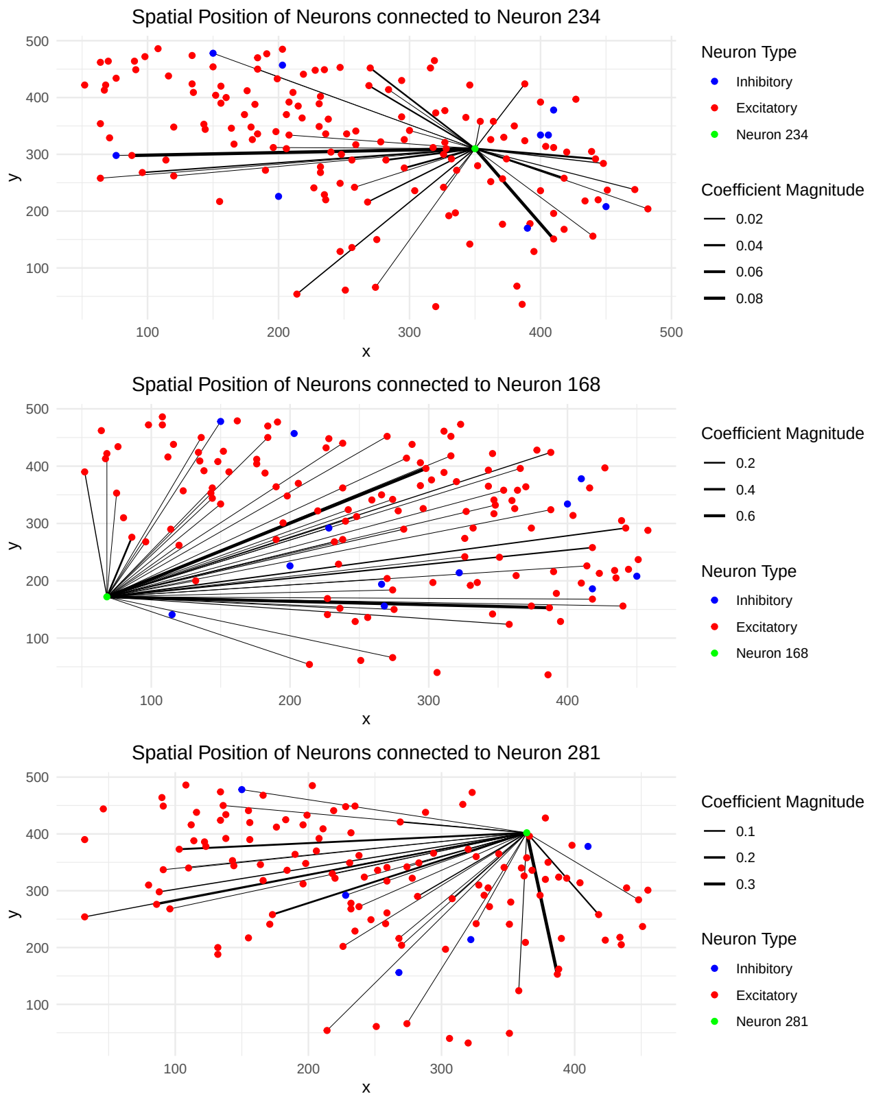
Figure 22: Predicted Neural Networks Using Best Model
