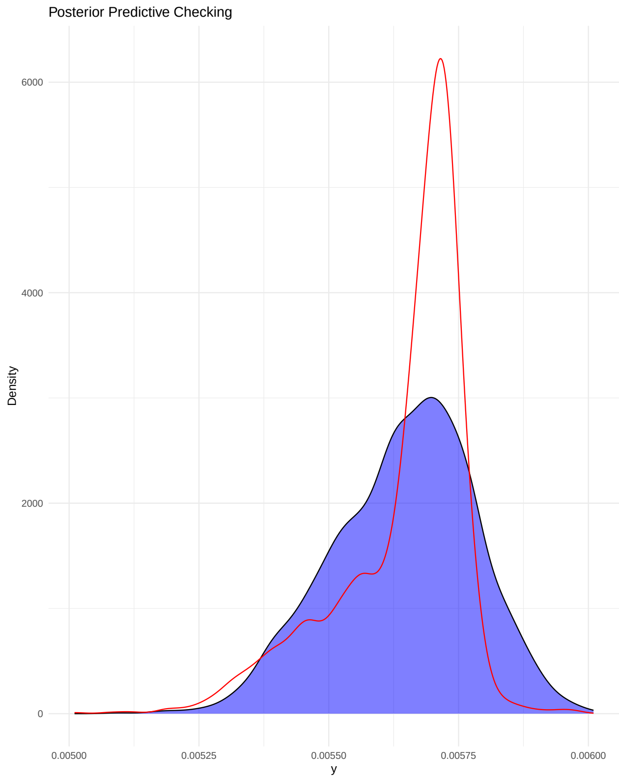
Figure 21: Posterior Predictive Checking for Best Bayesian Model
