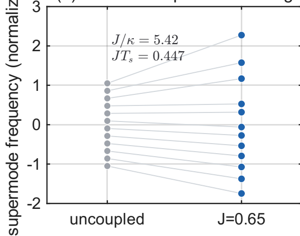
(b) Coherent supermode mixing
