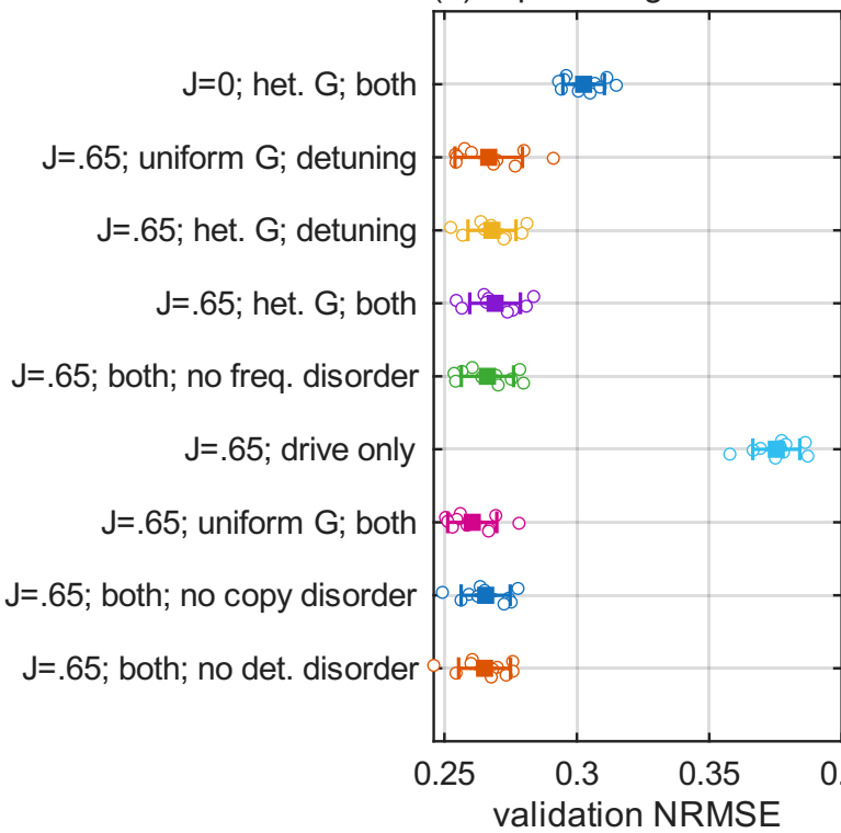
(a) Equal-budget ablations
