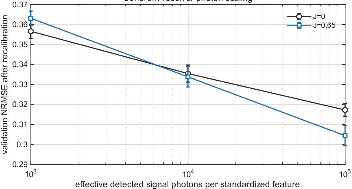
Coherent-receiver photon scaling
