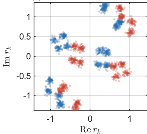
(c) ISI-distorted received field
