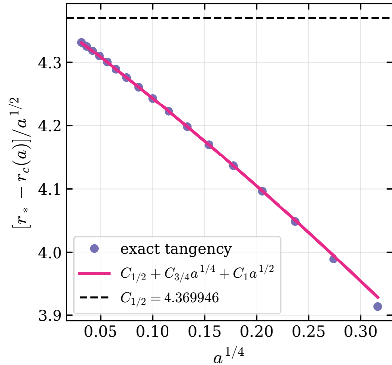
Second-order-EP scaling
