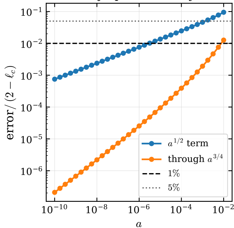
Asymptotic validity
