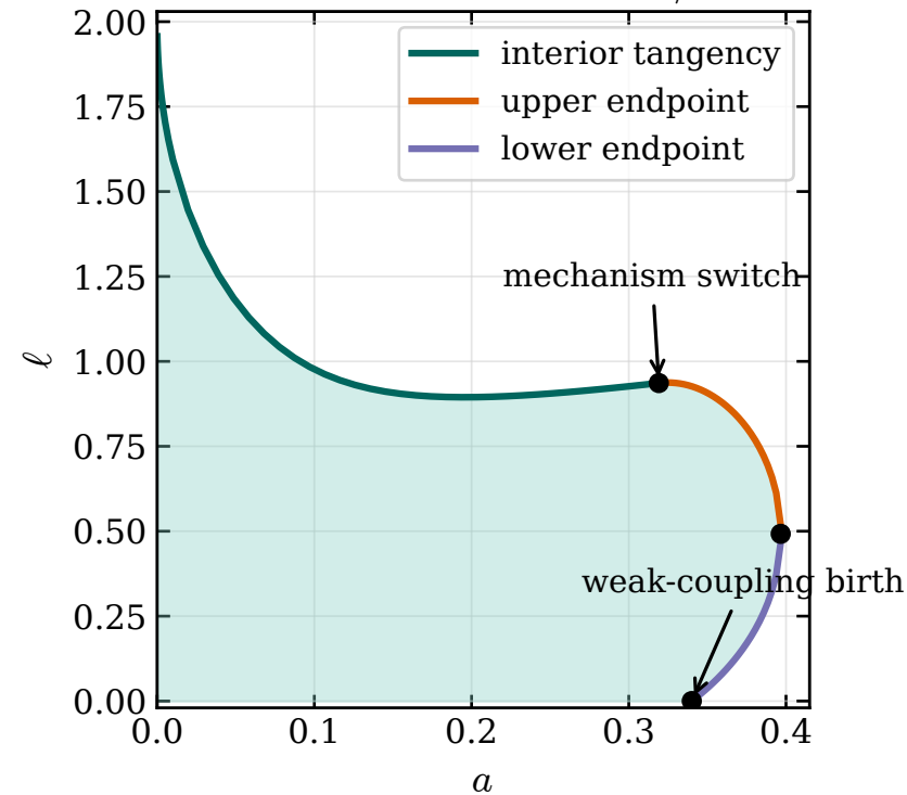
Resolved lobe ( \Omega_\Delta = 5/4 )
