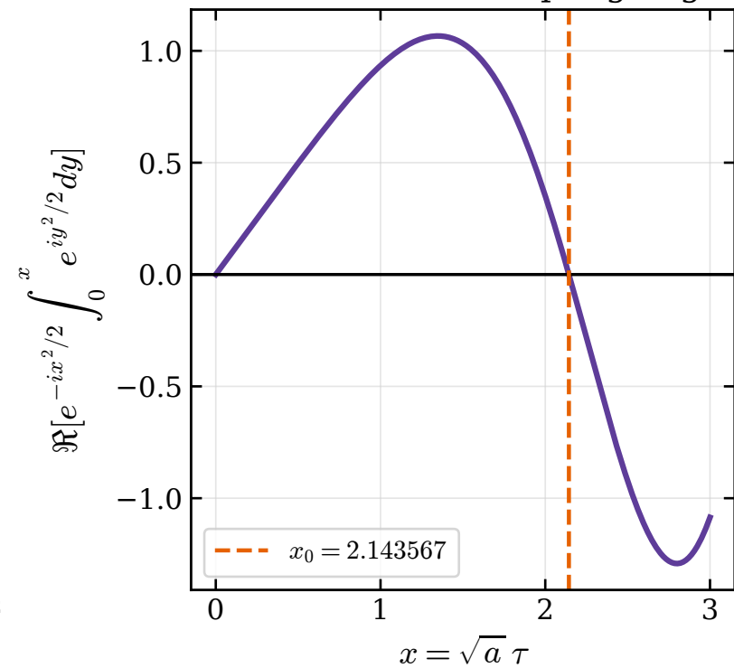
Universal weak-coupling edge
