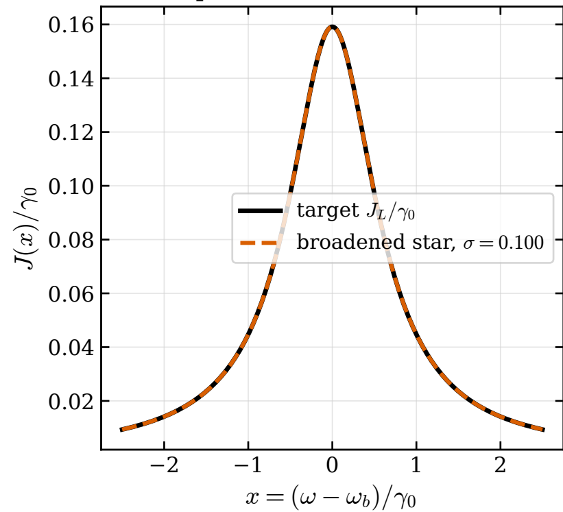
Spectral reconstruction
