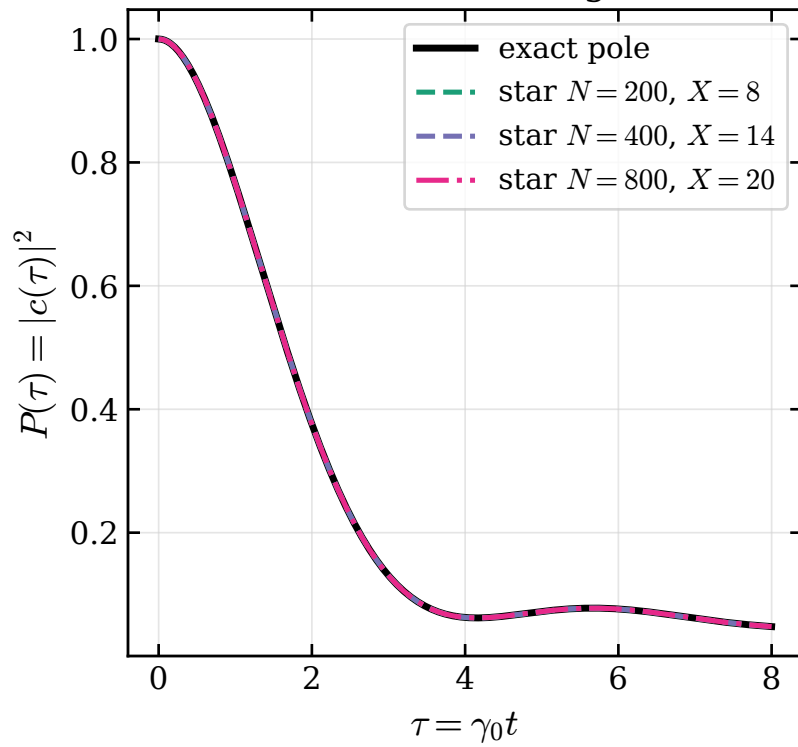
Continuum convergence
