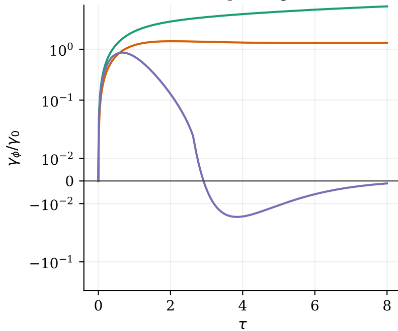
Exact dephasing rate
