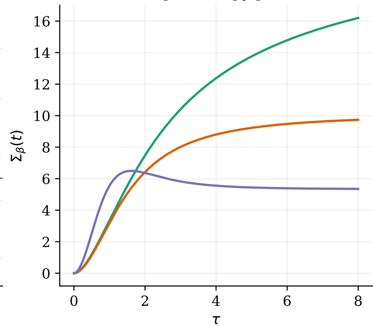
Microscopic entropy production
