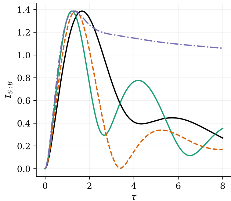
Vacuum correlations
