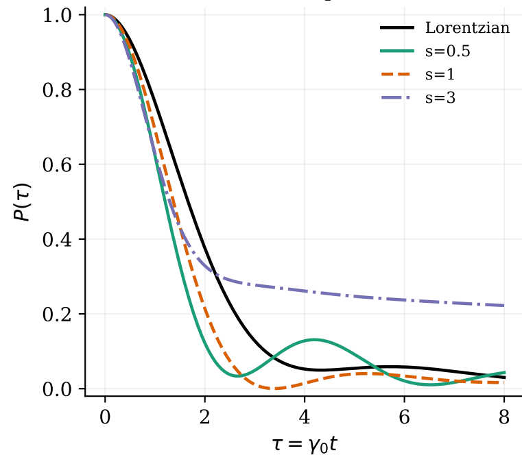
Bounded-chirp survival
