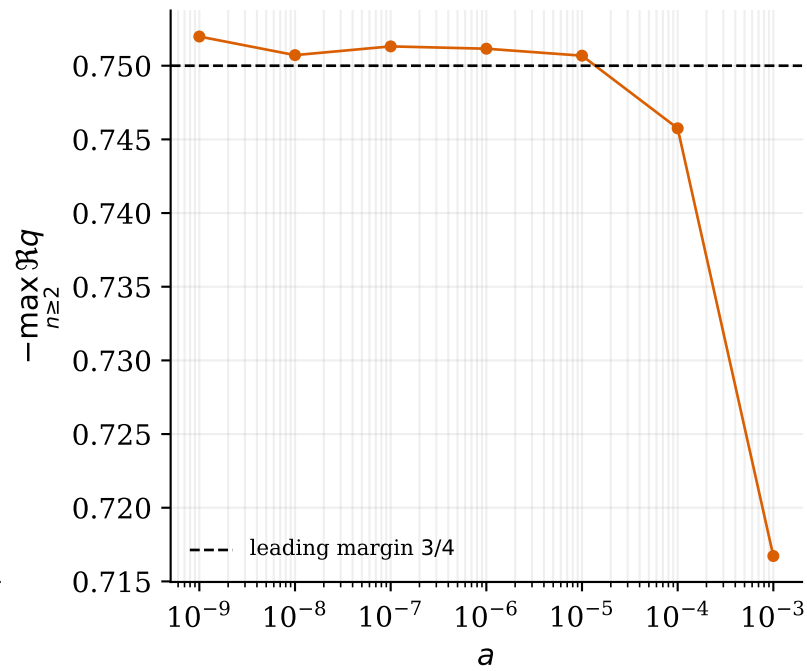
All later lifted zeros
