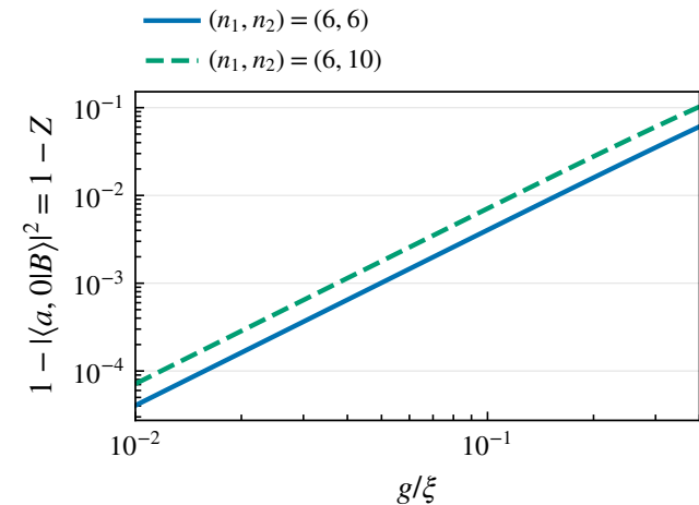
(c) Accuracy of the vacuum-field state
