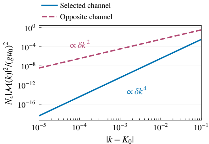
(c) Accuracy of the vacuum-field state
