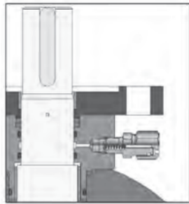
Stem Sealant Valve
