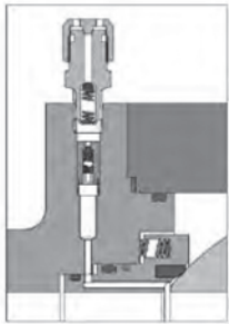
Seat Sealant Valve
