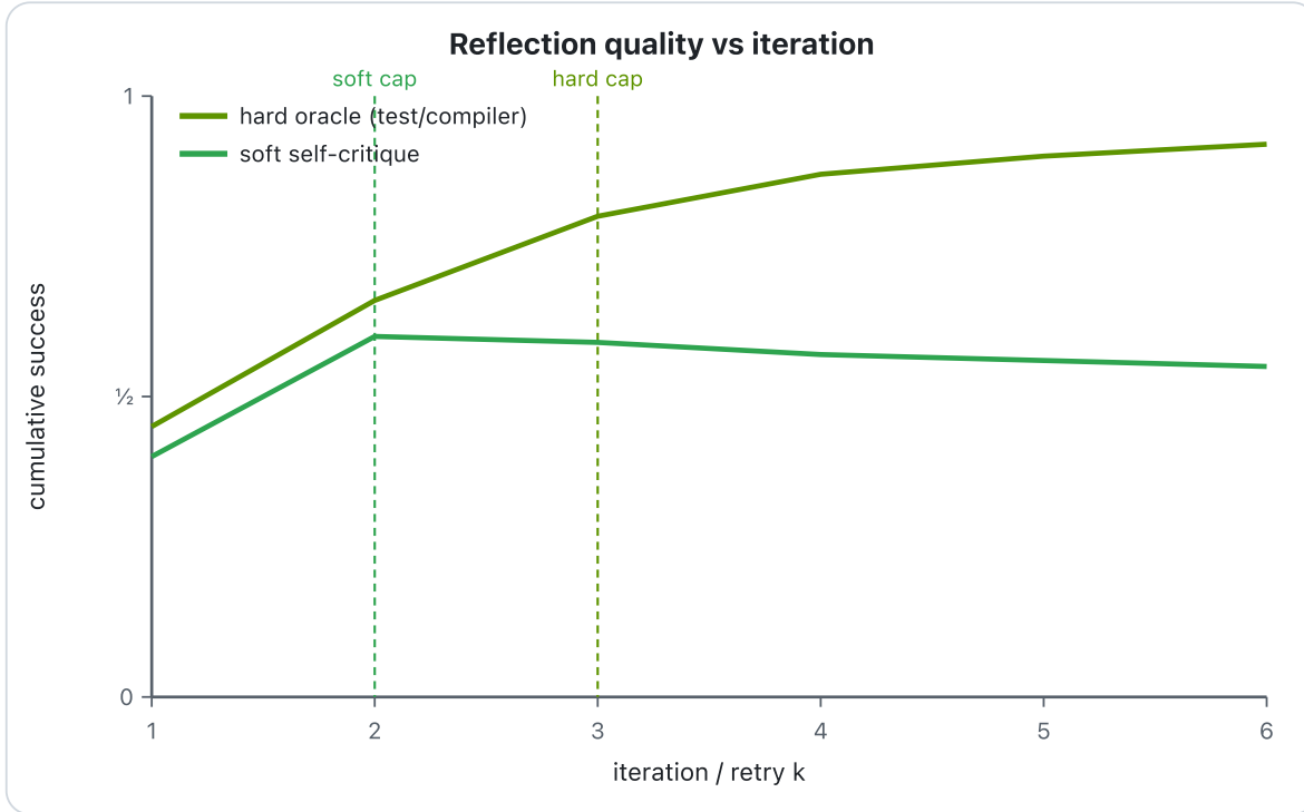
Figure 5. A hard oracle (test, compiler) keeps improving and saturates late; soft self-critique plateaus and dips after two passes (R8). The \sim 2 soft / \sim 3 hard caps are fabius's operational heuristics.
