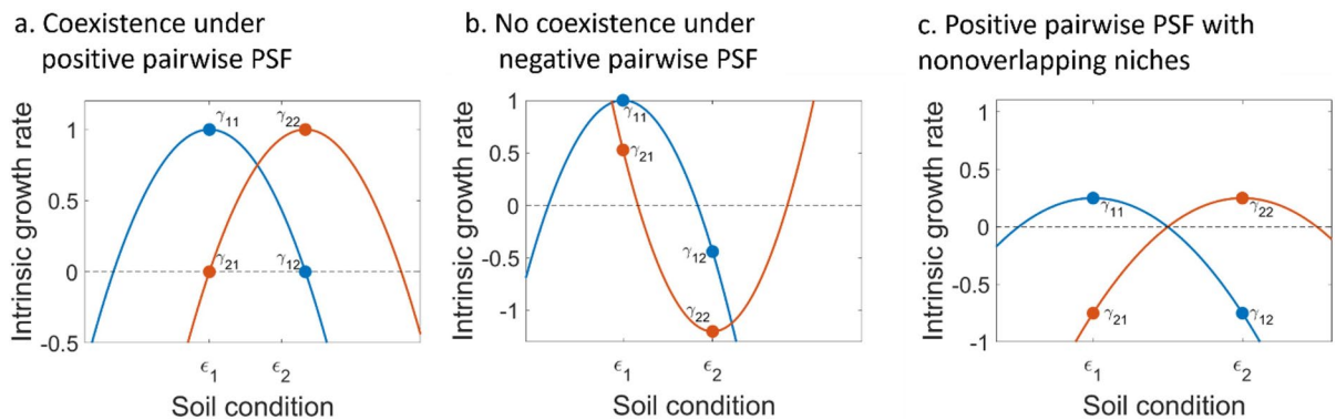
Fig. 2 Coexistence outcomes. Each panel shows the growth curves r(E) of species 1 (blue) and species 2 (orange). (a) Example where the current paradigm predicts exclusion, but our proposed framework shows that species coexist. (b) Example where the current paradigm predicts coexistence, but our proposed framework shows extinction of species 2. Here, the growth curve for species 2 has a local minimum between two peaks lying outside the displayed soil range. This can arise if
