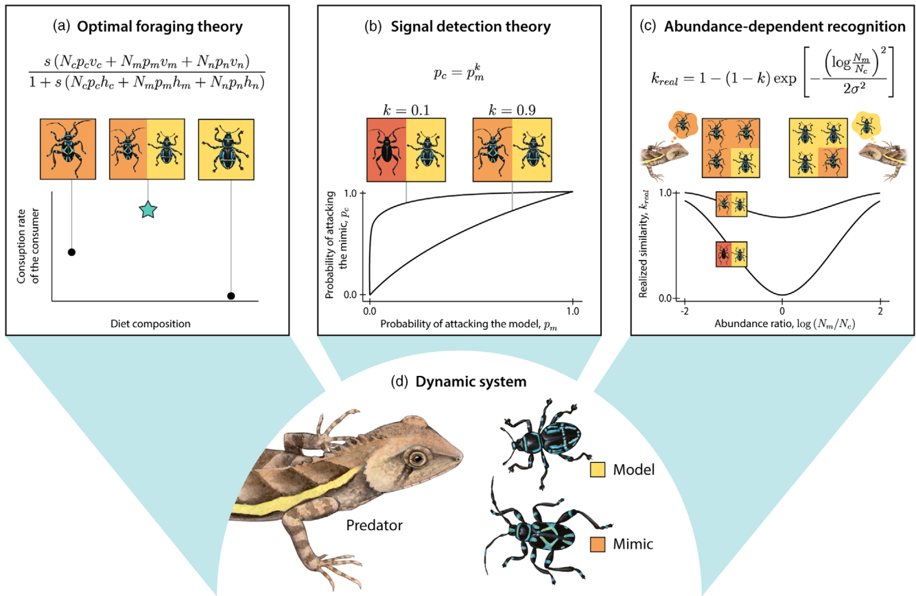
FIGURE 1 Illustrative figure demonstrating how our study incorporates (a) optimal foraging theory (i.e. predator optimizing attack probability p_i to maximize foraging gain), (b) signal detection theory (i.e. non-independence of attack probabilities via mimic-model morphological similarity k ), and (c) abundance-dependent recognition (i.e. predator realized recognition k_{real} also dependent of model-mimic abundance ratio) into a (d) dynamic system of mimic-model-predator. Here, only a single Batesian mimic is shown for simplicity (so the secondary subscript j in N_c is omitted). In panels (b) and (c), we depict two scenarios with low ( k = 0.1 ; red mimic) and high ( k = 0.9 ; orange mimic) innate mimic-model morphological similarity k . See the main text for the mathematical description of the full multi-mimic model. This figure is illustrated by Julie Johnson from Life Science Studios.
