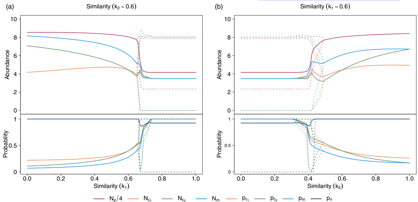
FIGURE 5 Bifurcation plot of the multi-mimicry system. (a) bifurcation along the Batesian mimic–model morphological similarity ( k_1 ) while fixing the Müllerian mimic's morphological similarity ( k_2 = 0.6 ). (b) bifurcation along the k_2 while fixing k_1 = 0.6 . The y-axis of the upper panels shows abundance, and the lower panels show the attack probability. The upper panels of both plots illustrate the abundances of the predator ( N_p ; red), the Batesian mimic ( N_{c1} ; orange), the Müllerian mimic ( N_{c2} ; green) and the model ( N_m ; light blue). Note that the abundance of the predator is divided by four for better visualization. The lower panels of both plots illustrate the predator's attack probability on the Batesian mimic ( p_{c1} ; orange), the Müllerian mimic ( p_{c2} ; green), the model ( p_m ; light blue) and the alternative prey ( p_n ; dark blue). The solid and dashed lines in all panels represent the mean and maximum/minimum values, respectively.
