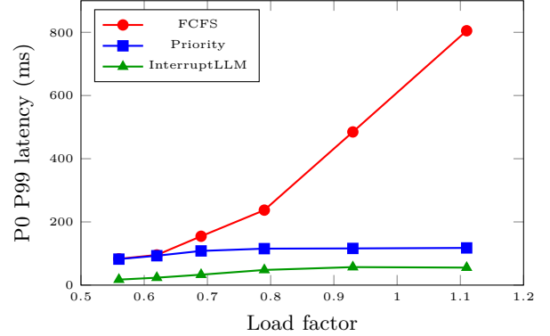
Fig. 2: P0 P99 latency vs. load factor.
