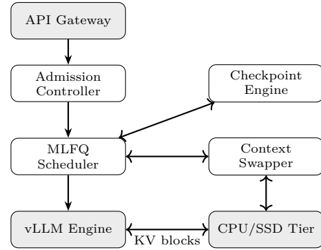
Fig. 1: InterruptLLM architecture.
