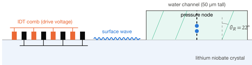
Figure 3: The device in cross-section. A comb-shaped electrode drives a ripple along the crystal surface. Because the ripple travels faster in the crystal ( 3979\text{ m/s} ) than sound does in water ( 1497\text{ m/s} ), it leaks into the liquid at a fixed angle of about 22^\circ — the same reason a straw looks bent in a glass of water. Two such waves sent from opposite sides make the standing pattern.
