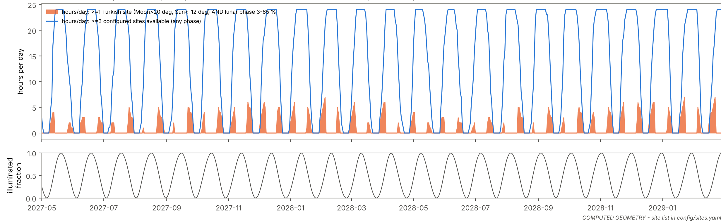
Observer availability over the impact-epoch domain (seasonal closures included); lower panel: lunar phase
