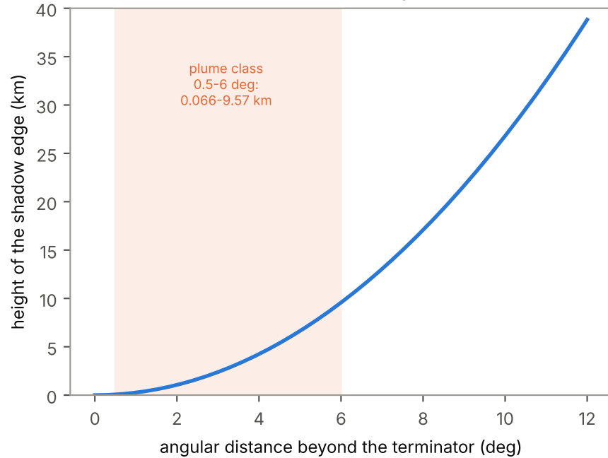
b) Height ejecta must reach to be sunlit (point Sun, sphere; the finite solar disc and terrain broaden the edge)
