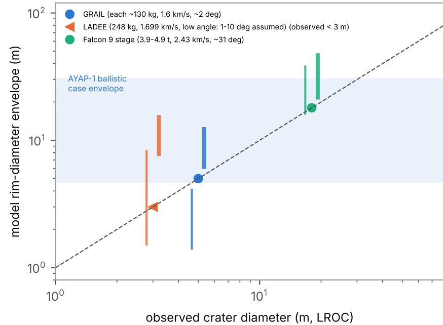
c) Consistency check, no tuning (thin: vertical-component rule; thick: vertical-equivalent; parameter sets x densities 150-1000)
