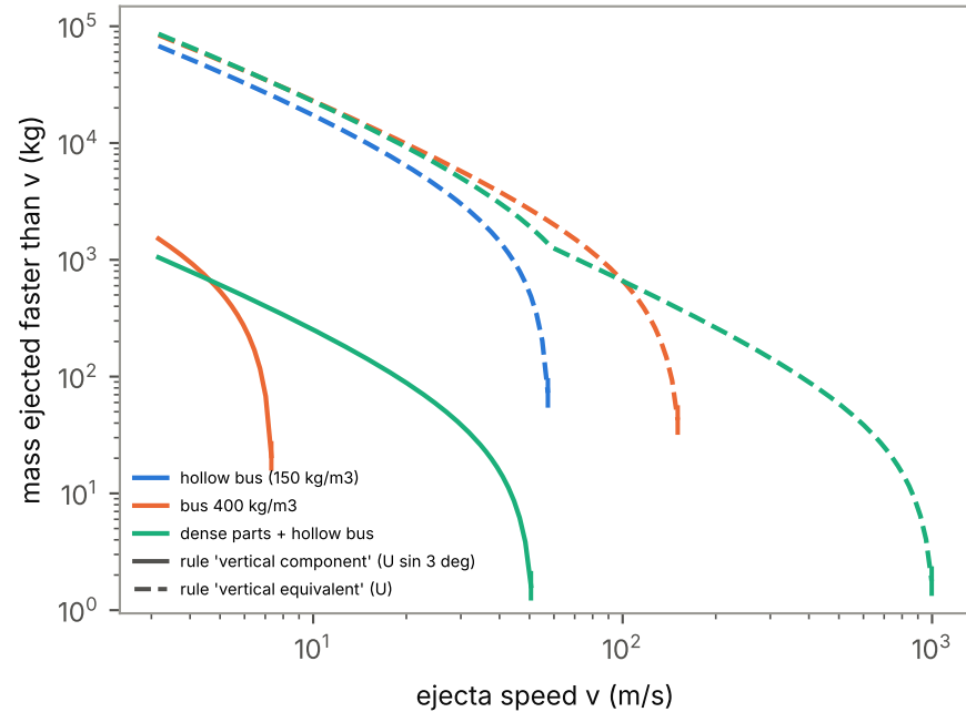
a) Ejecta mass-speed, ballistic case (HH2011, sand); curves stop at the scaling-domain edge (bar): faster = cannot determine
