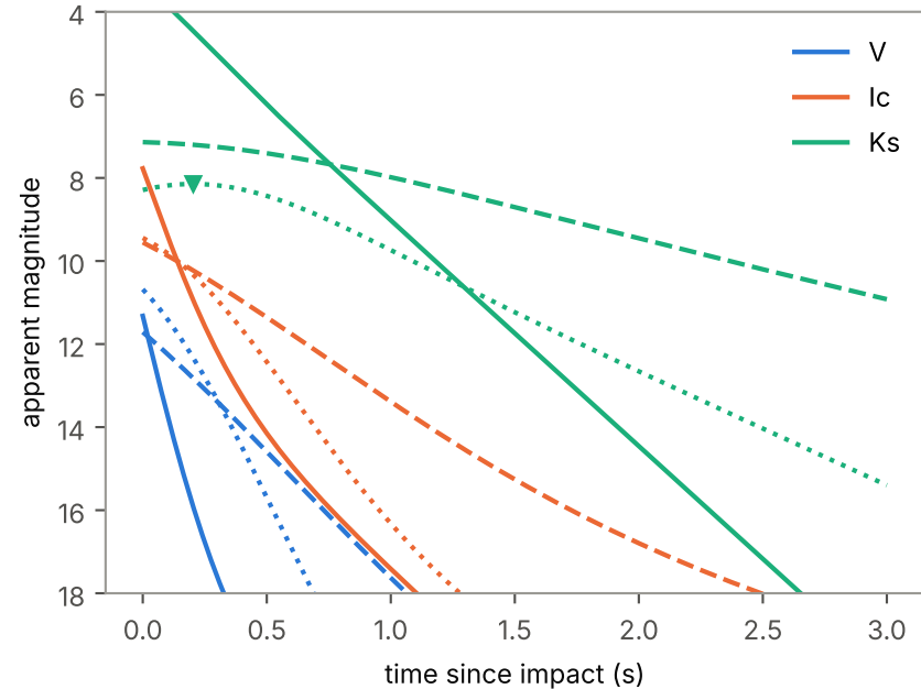
a) Light curves, \eta_{\text{vis}} 1e-4 (solid 2000 K, 0.2 s; dashed 3000 K, 0.8 s; dotted 4500 K, 0.4 s); triangles: delayed band peaks
