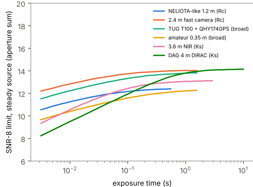
c) Above-atmosphere limits vs exposure (illum 0.35, 8' from sunlit terrain, airmass 1.2; lines end where the background passes half full well)
