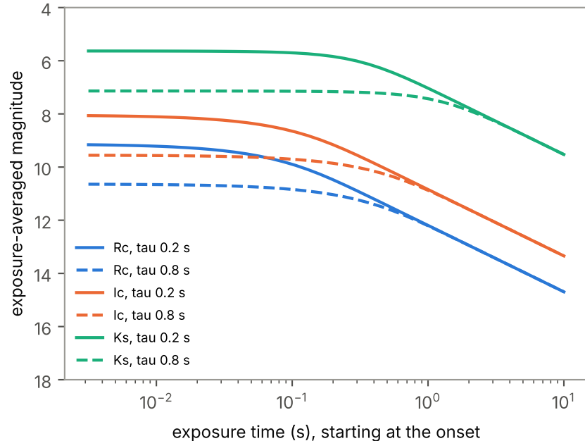
b) Dilution of the flash in longer exposures (T0 3000 K)
