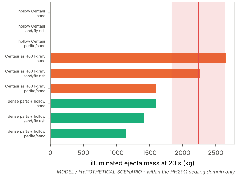
c) LCROSS like-for-like check (observed 2240 +/- 400 kg, Strycker et al. 2013): a calibration of the bulk density, not a validation
