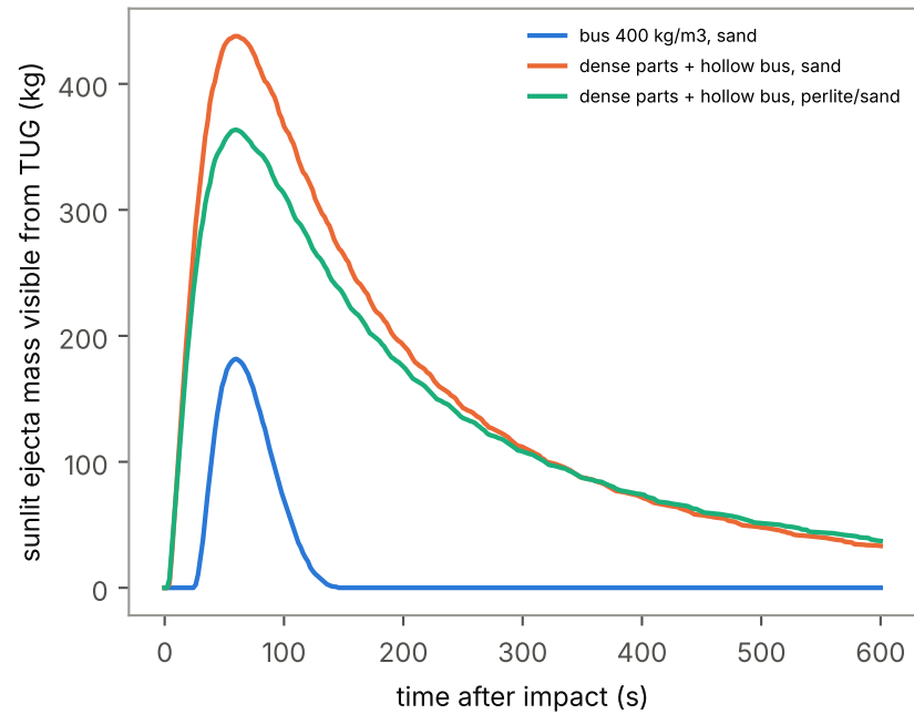
a) S2 (3.3 deg beyond the terminator, shadow edge 2.9 km): sunlit ejecta mass, rule 'vertical equivalent' (the other rule: cannot determine)
