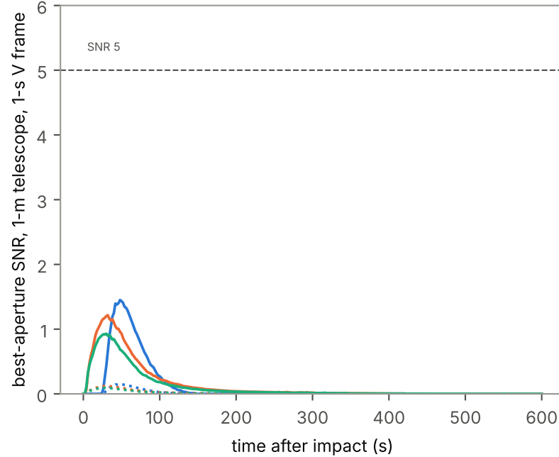
b) Plume signal-to-noise against the total background (solid: subtraction systematic 1e-3; dotted: 1e-2)
