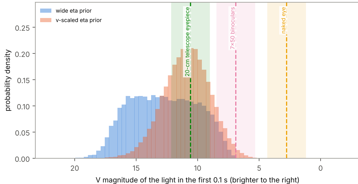
a) Visual-threshold model, S1 at Istanbul (Moon 53 deg, 39 % lit); bands: field factor 1.4-24; conditional on a clear, unobstructed, attentive view
