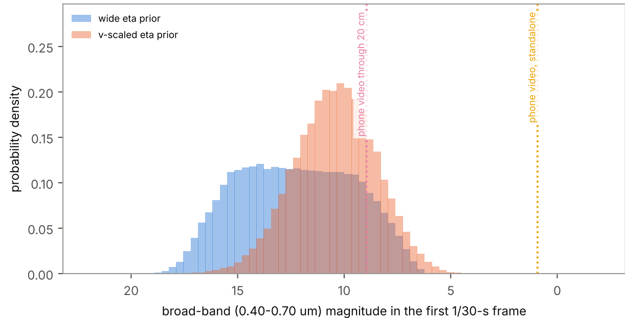
b) Phone video limits (SNR 8 after the declared processing penalty), broad band: not V magnitudes; not comparable with panel a without colour terms
