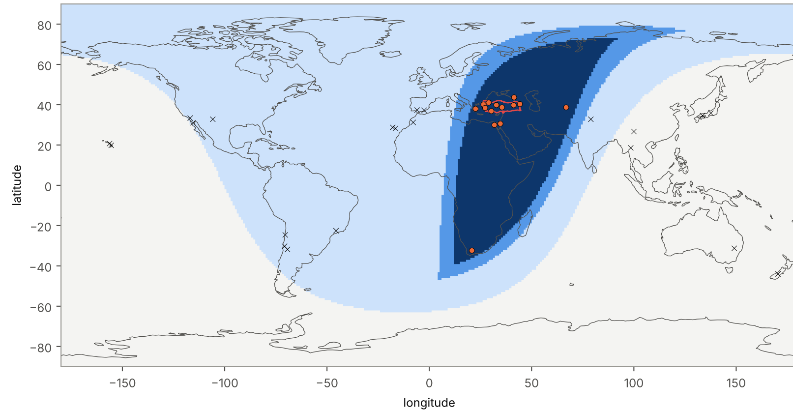
S10: Earth coverage at the impact time 2028-04-01 18:00 UTC (2028-04-01 21:00 in Türkiye, UTC+3)
