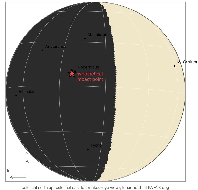
Moon from Earth's centre: illuminated 39 %
