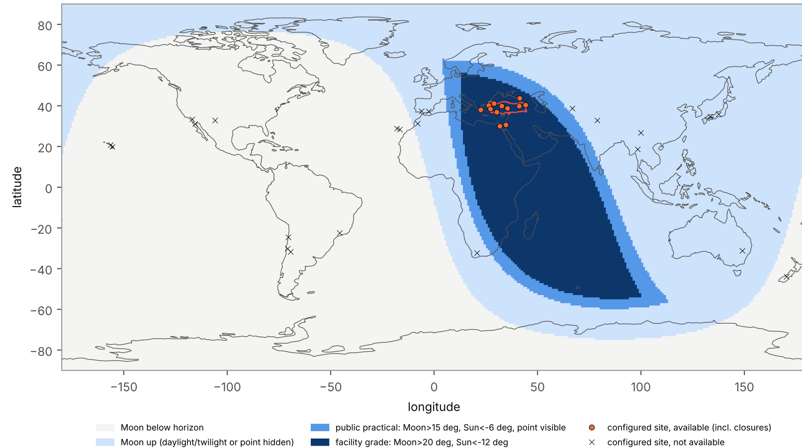
S3: Earth coverage at the impact time 2028-07-15 00:00 UTC (2028-07-15 03:00 in Türkiye, UTC+3)
