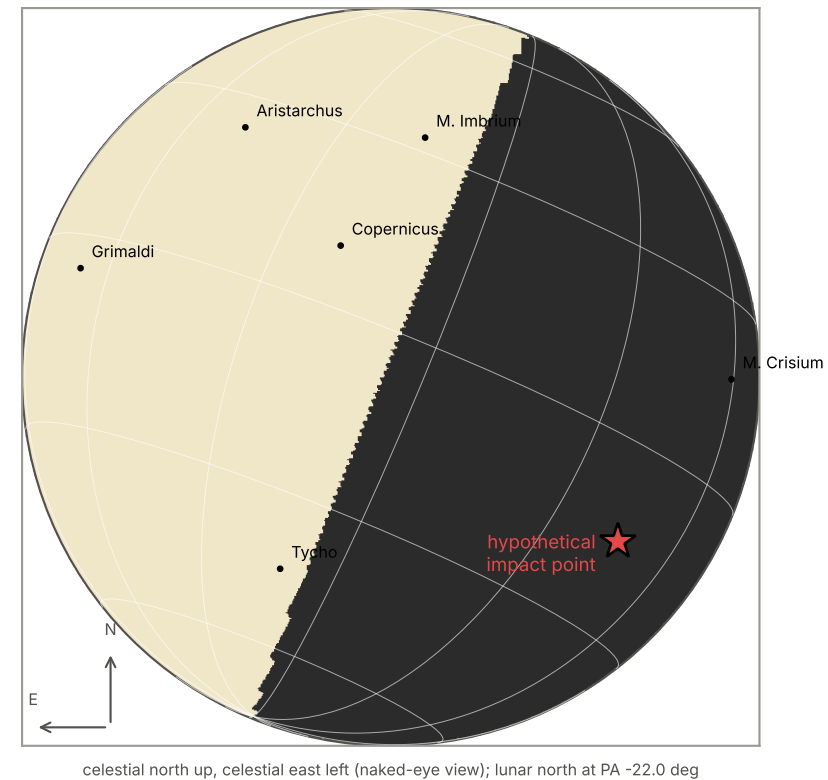
Moon from Earth's centre: illuminated 49 %
