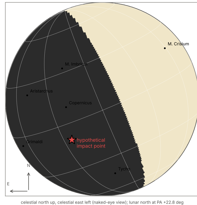
Moon from Earth's centre: illuminated 42 %
