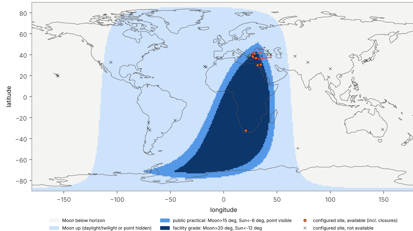
S4: Earth coverage at the impact time 2028-06-28 19:00 UTC (2028-06-28 22:00 in Türkiye, UTC+3)
