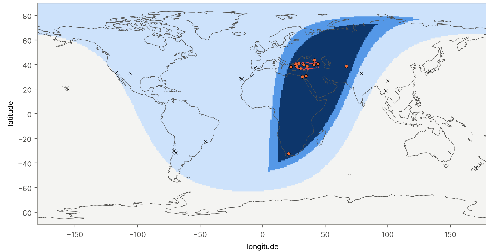
S7: Earth coverage at the impact time 2028-04-01 18:00 UTC (2028-04-01 21:00 in Türkiye, UTC+3)
