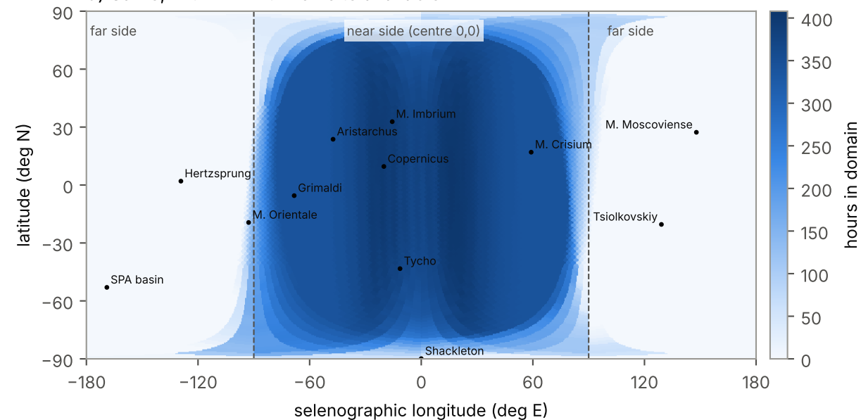
d) Same, with >= 1 Turkish site available
