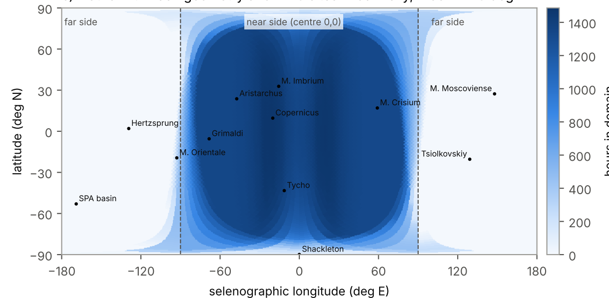
c) Hours with flash geometry and >= 3 sites in dark sky, Moon > 20 deg
