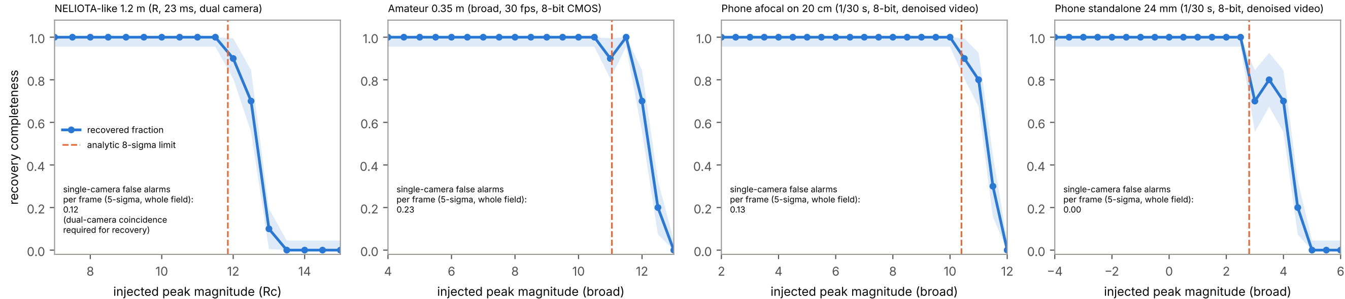
Injection-recovery on synthetic lunar video (SIMULATION; illuminated fraction 0.35, flash durations 0.1-1 s, 5-sigma matched filter; shaded: binomial 1-sigma)
