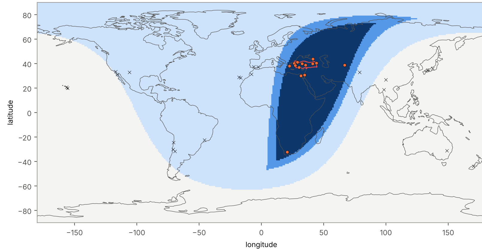
S1: Earth coverage at 2028-04-01 18:00 UTC, 2028-04-01 21:00 in Türkiye (UTC+3)
